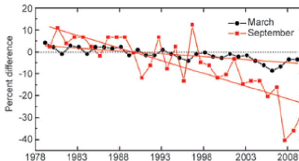
FIG. 5.12. Time series of the percent difference in ice extent in March (the month of ice extent maximum) and September (the month of ice extent minimum) relative to the mean values for the period 1979–2000. Based on a least squares linear regression for the period 1979–2009, the rate of decrease for the March and September ice extents is -2.5\% and -8.9\% per decade, respectively.
